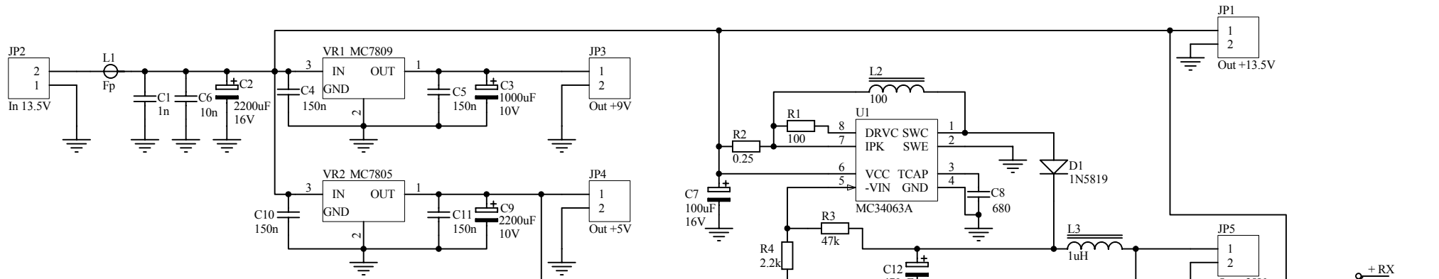
Voltages, VOX and RX/TX commutation for VCODDS v1.0 by Ivan Dachev and LZ2GL
