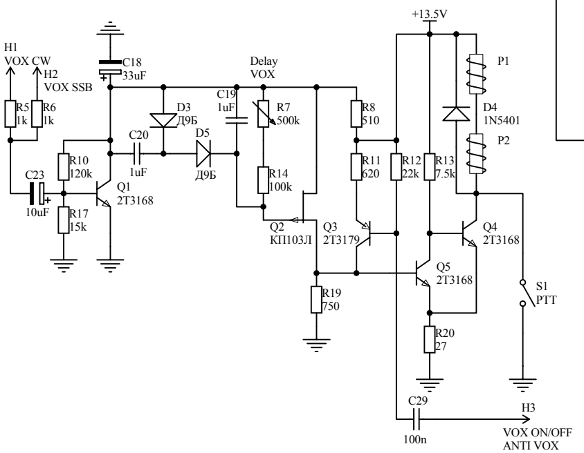
Voltages, VOX and RX/TX commutation for VCODDS v1.0 by Ivan Dachev and LZ2GL
