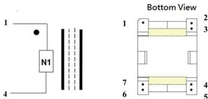
Figure 9. Transformer Specifications & Construction
