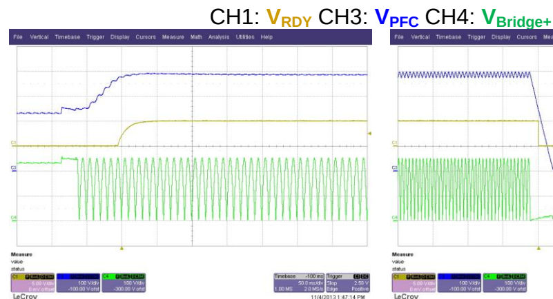
Figure 13. PFC ON
