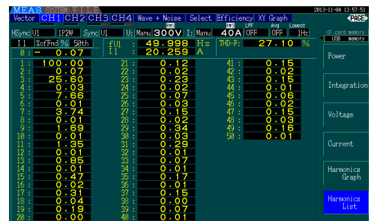
Figure 28. 100% Load
