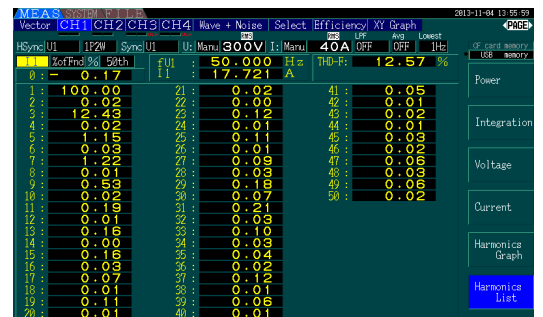
Figure 23. 75% Load
