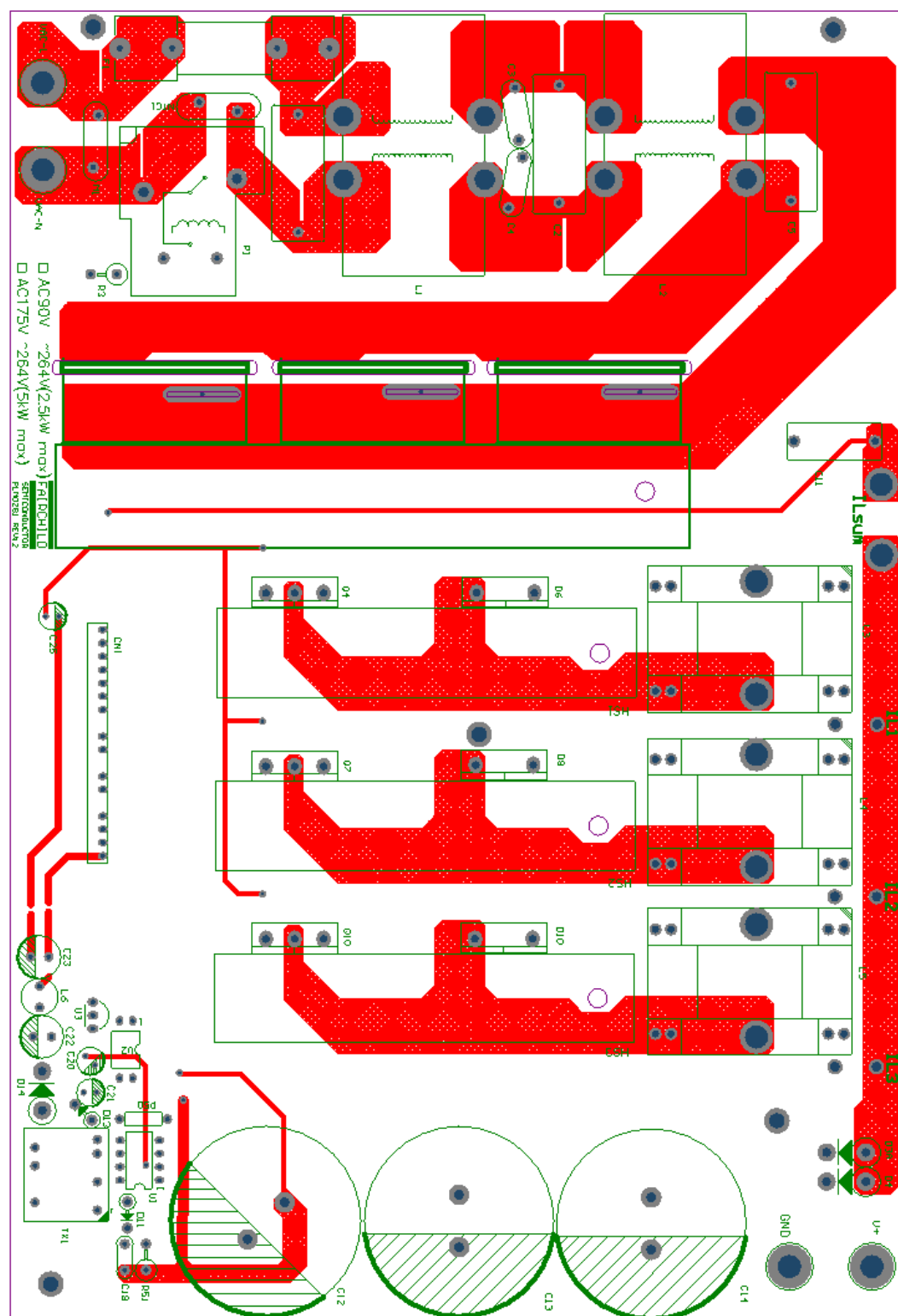
Figure 2. Top Side of Evaluation Board
