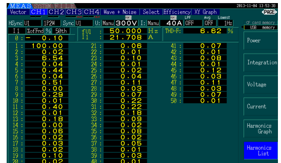
Figure 19. 75% Load
