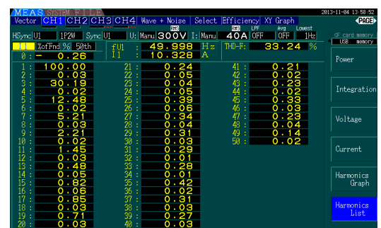
Figure 26. 50% Load
