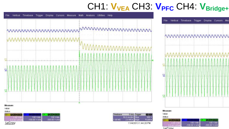
Figure 11. 180 V→264 V 5000 W Load
