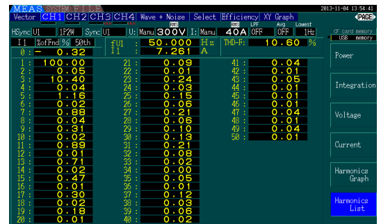
Figure 17. 25% Load
