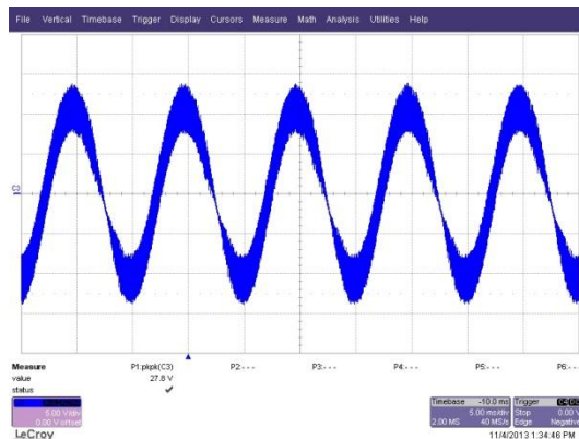
Figure 15. 180 V / 50 Hz
