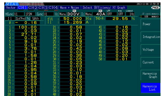
Figure 27. 75% Load
