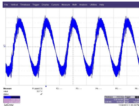
Figure 16. 264 V / 50 Hz
