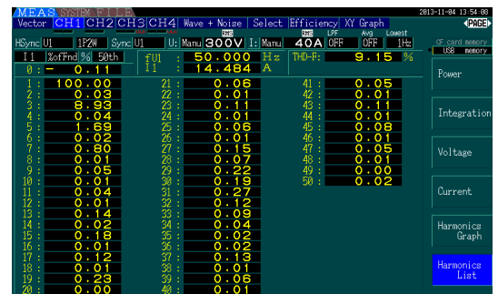
Figure 18. 50% Load
