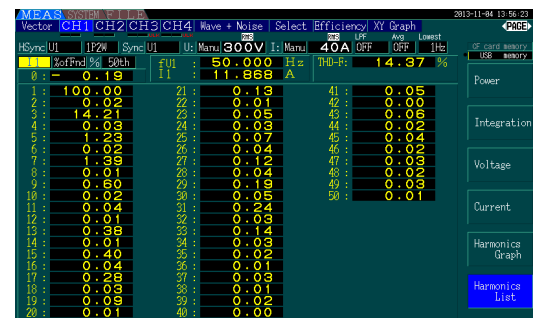
Figure 22. 50% Load
