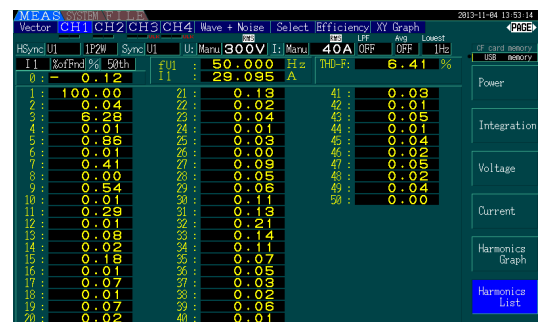
Figure 20. 100% Load
