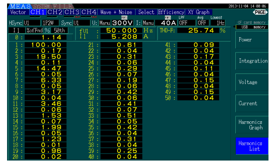
Figure 25. 25% Load
