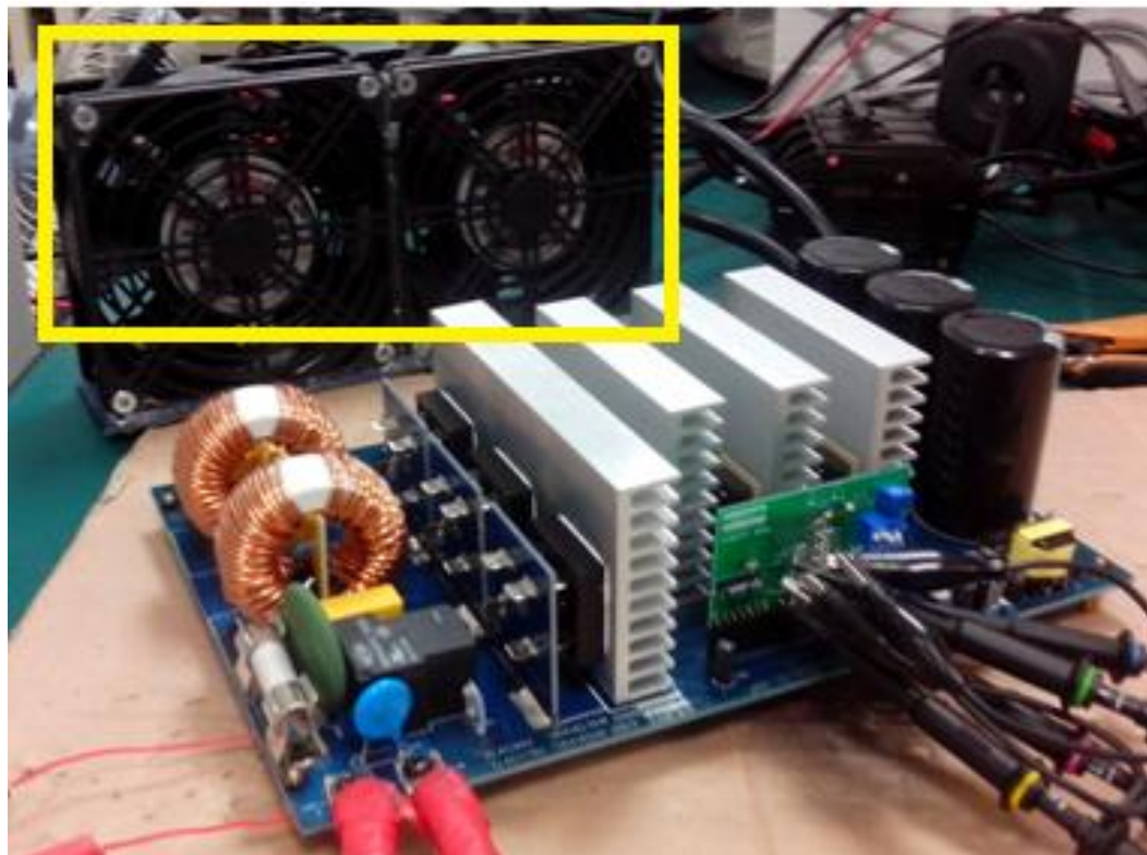
Figure 29. Recommended Fan Setup
