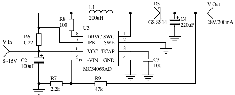
Encoders and Voltage Step-Up converter for VCODDS v1.0 by Ivan Dachev and LZ2GL
